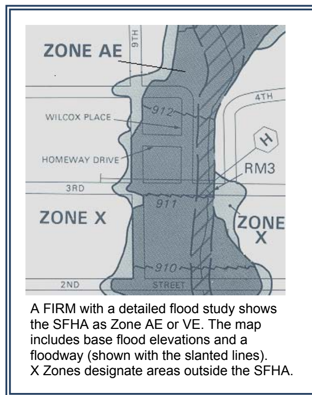
Figure 410-1. FIRM terminology.
